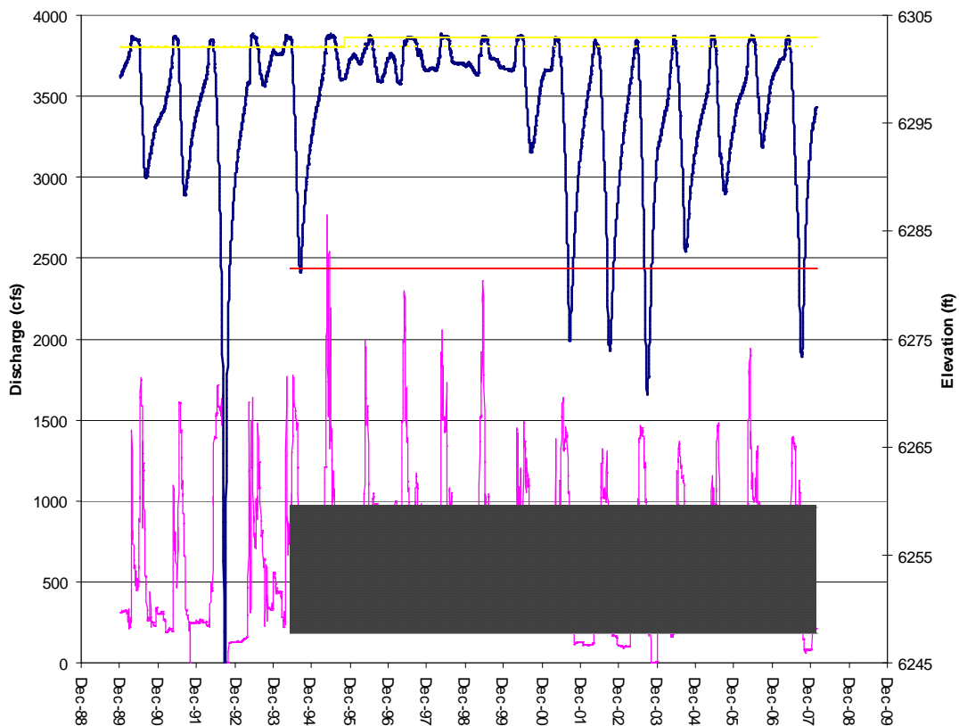
Figure 13. Island Park Reservoir water surface elevation (heavy blue) and discharge (magenta). Since it began operating in June of 1994, discharges between 180 and 960 cfs (gray rectangle) are passed through the Island Park Hydro-electric plant, except when water surface elevation drops below 6281.5 (red line) when the siphon ceases to function and all the water passes through the unscreened gates. At elevations above 6202 ft spill occurred prior to 1995, when a rubber collar was installed on the spillway and allows regulation of spill between 6302 and 6303 elevation (dotted and solid yellow lines).
