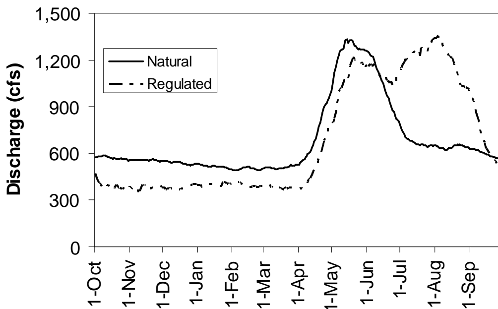
Figure 2. Mean natural and regulated flow at Island Park Dam, 1972 - 2003 (from Van Kirk and Burnett 2004).
