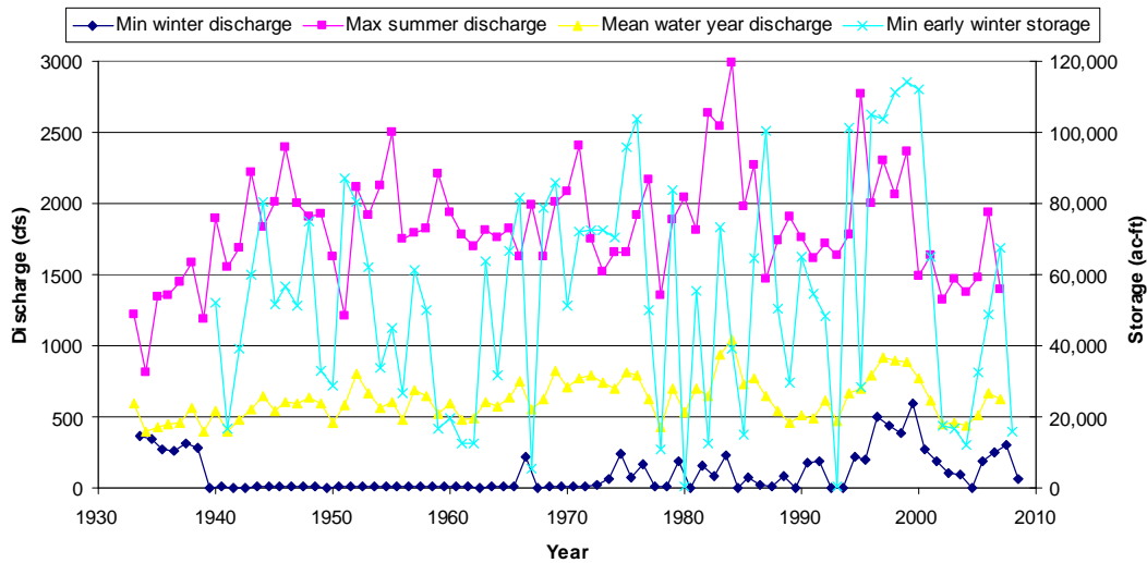
Figure 3. Minimum early winter (September - December) storage volume in Island Park Reservoir, along with minimum winter (October - March), maximum summer (April - September) and mean water year (October - September) discharge in the Henrys Fork downstream from Island Park Dam (mean discharge for the period of record is 620 cfs).
